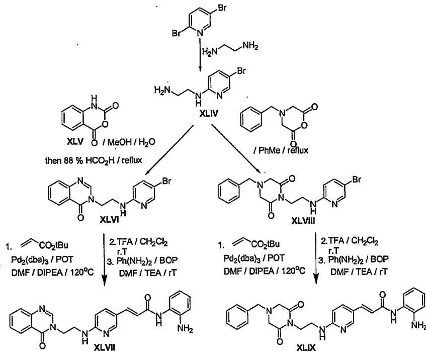
Scheme 8
